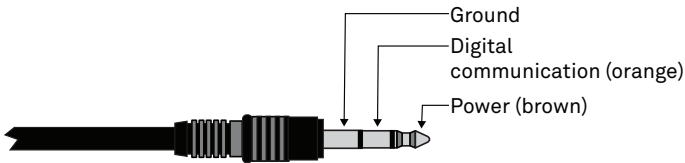
Figure 1 Stereo plug connector
